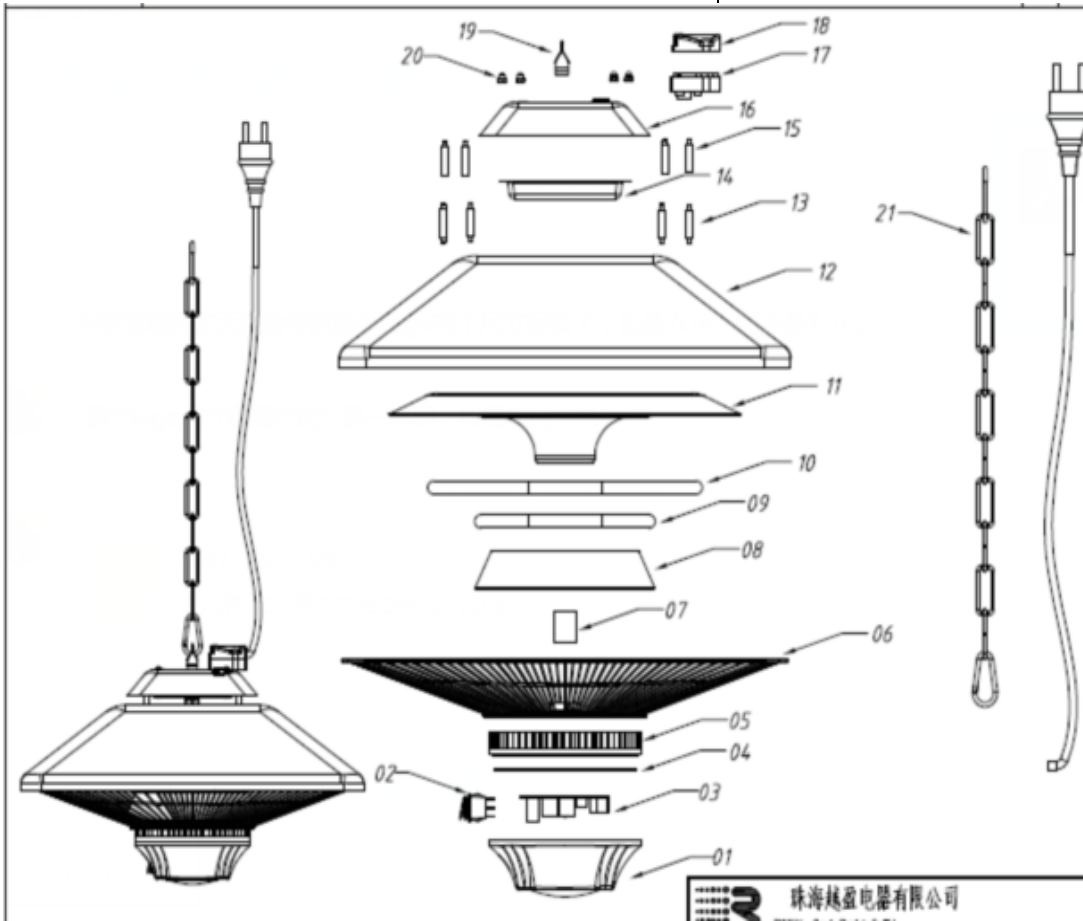
ZHQ2088-RMLED-II Explode Drawing
